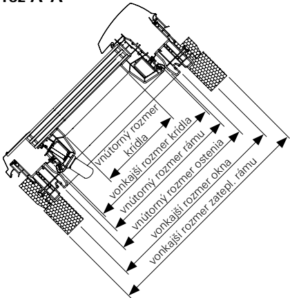
rez A–A
